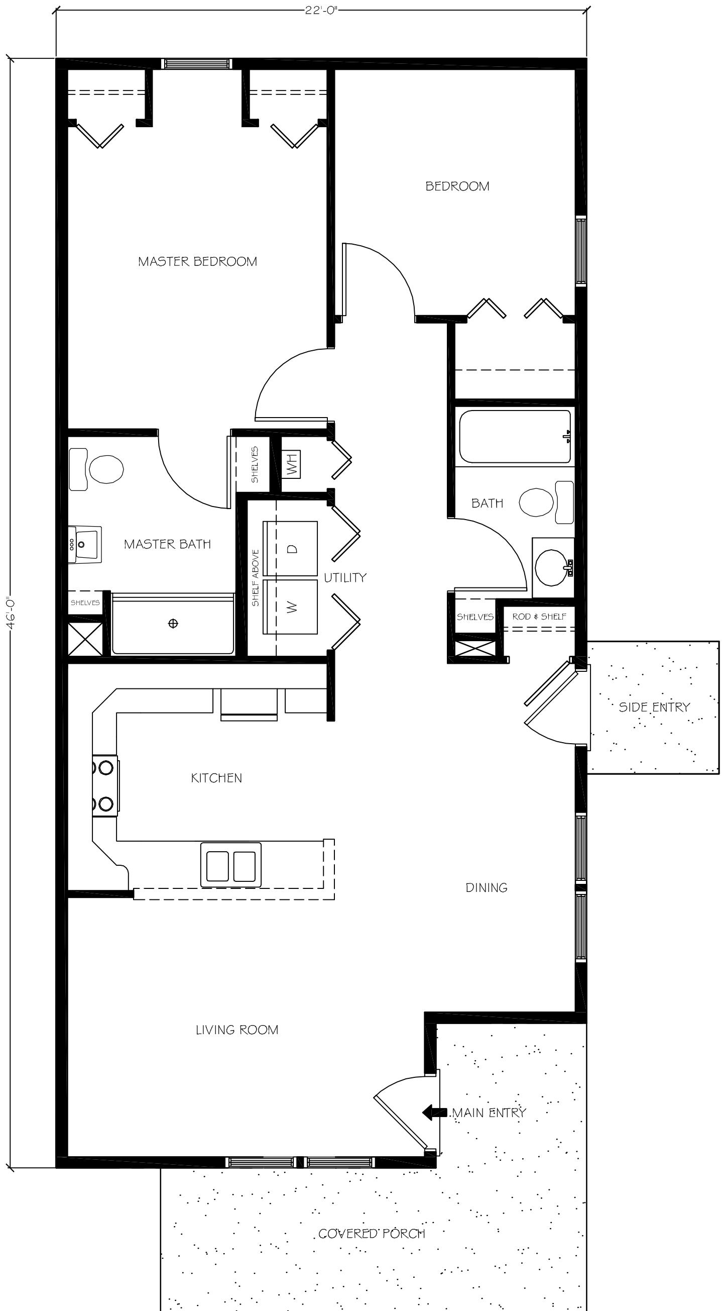
1 HABITAT FLOOR PLAN (2014) A1.0 SCALE: 1/4" = 1'-0"
